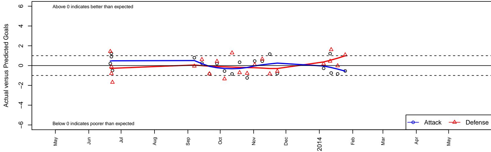
North Whidbey Islanders G99 Dots are actual minus expected GF (blue circles) and GA (red triangles). Blue line is smoothed change in attack strength. Red is smoothed change in defense strength.
